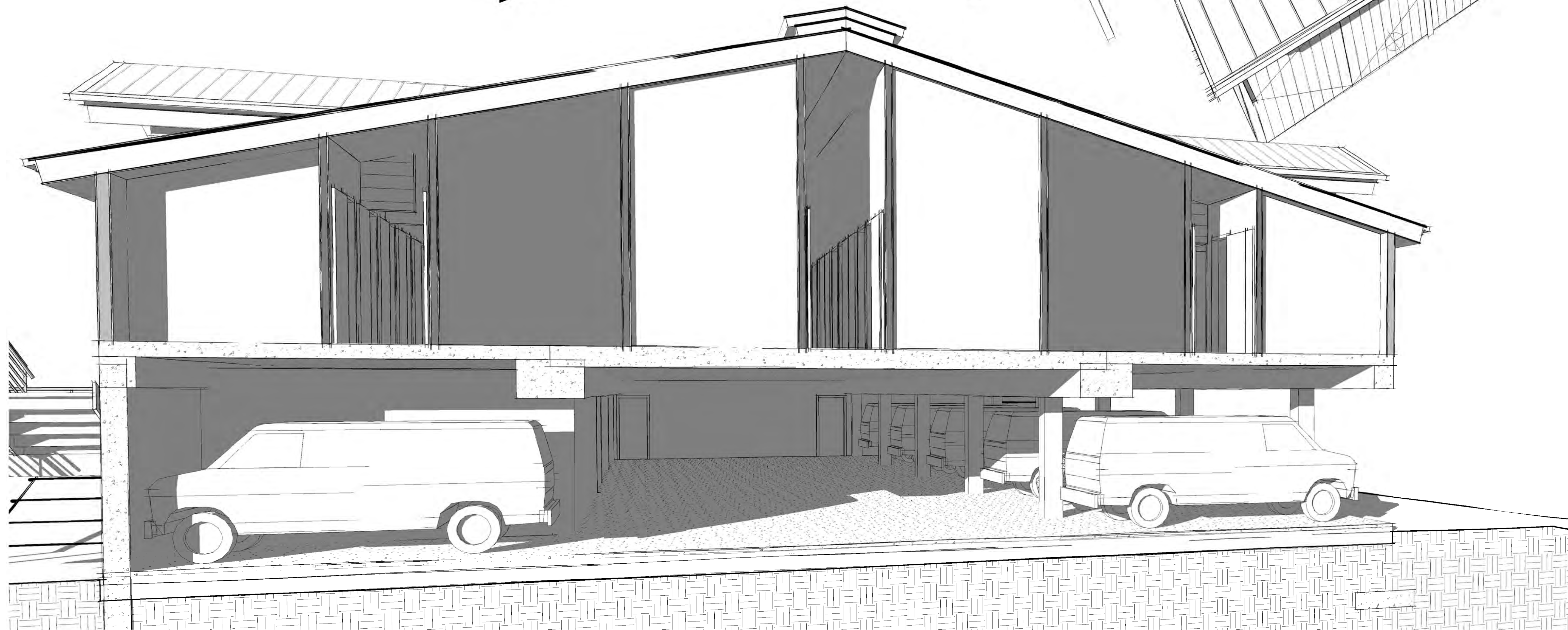
2 3D SECTION 1 A901 OPTION: GABLE DORMERS
