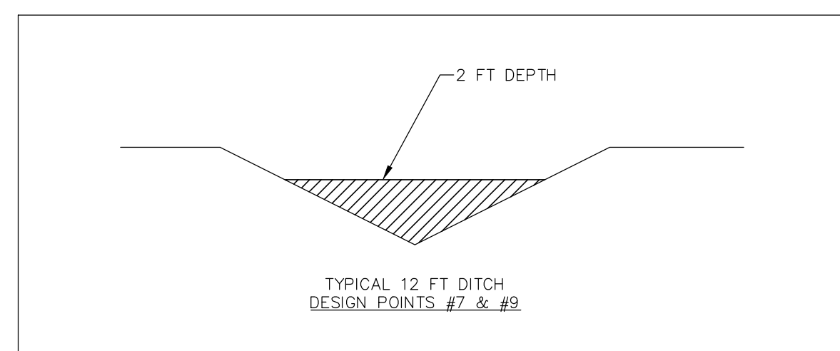
DITCH CONVEYANCE
