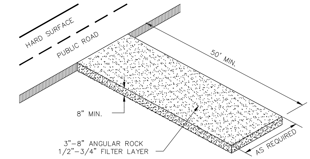
VEHICLE TRACKING CONTROL DETAIL NOT TO SCALE
