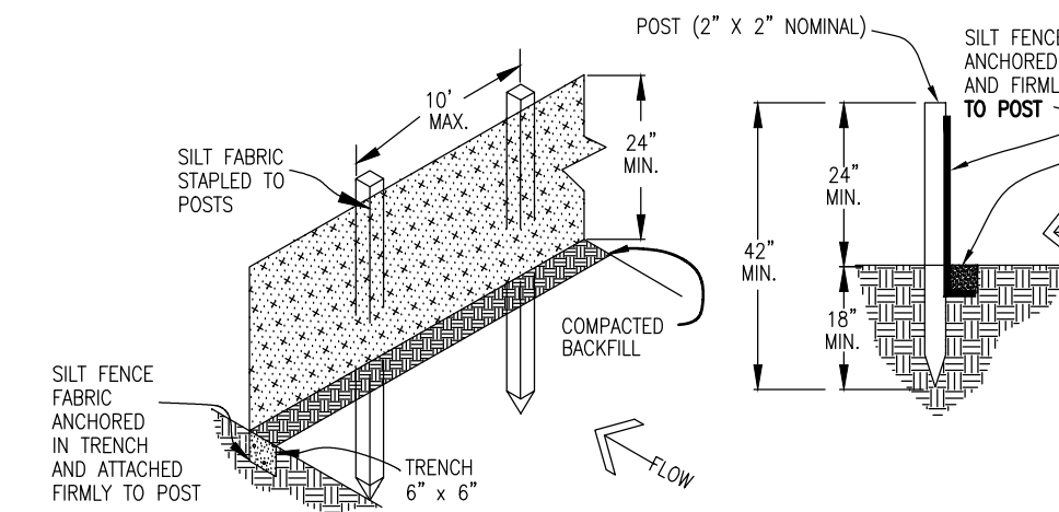
SILT FENCE DETAILS NOT TO SCALE
