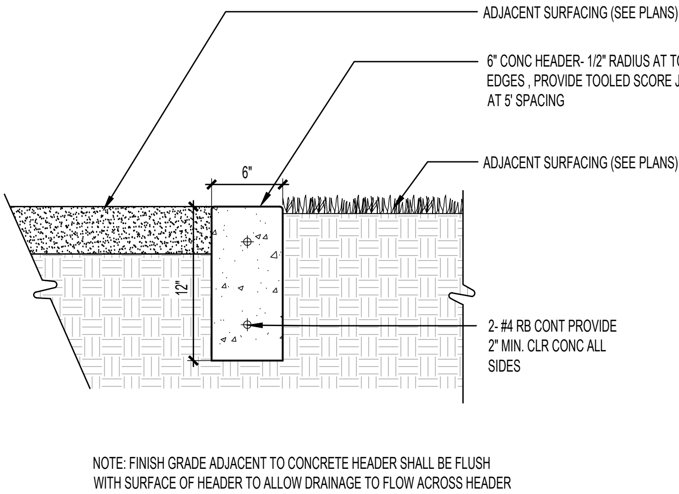
D FLUSH CONCRETE HEADER SCALE: 1/12" = 1'-0"
