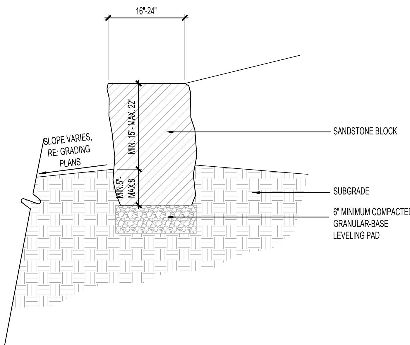
E DECORATIVE LANDSCAPE BOULDER SCALE: 1/4" = 1'-0"
