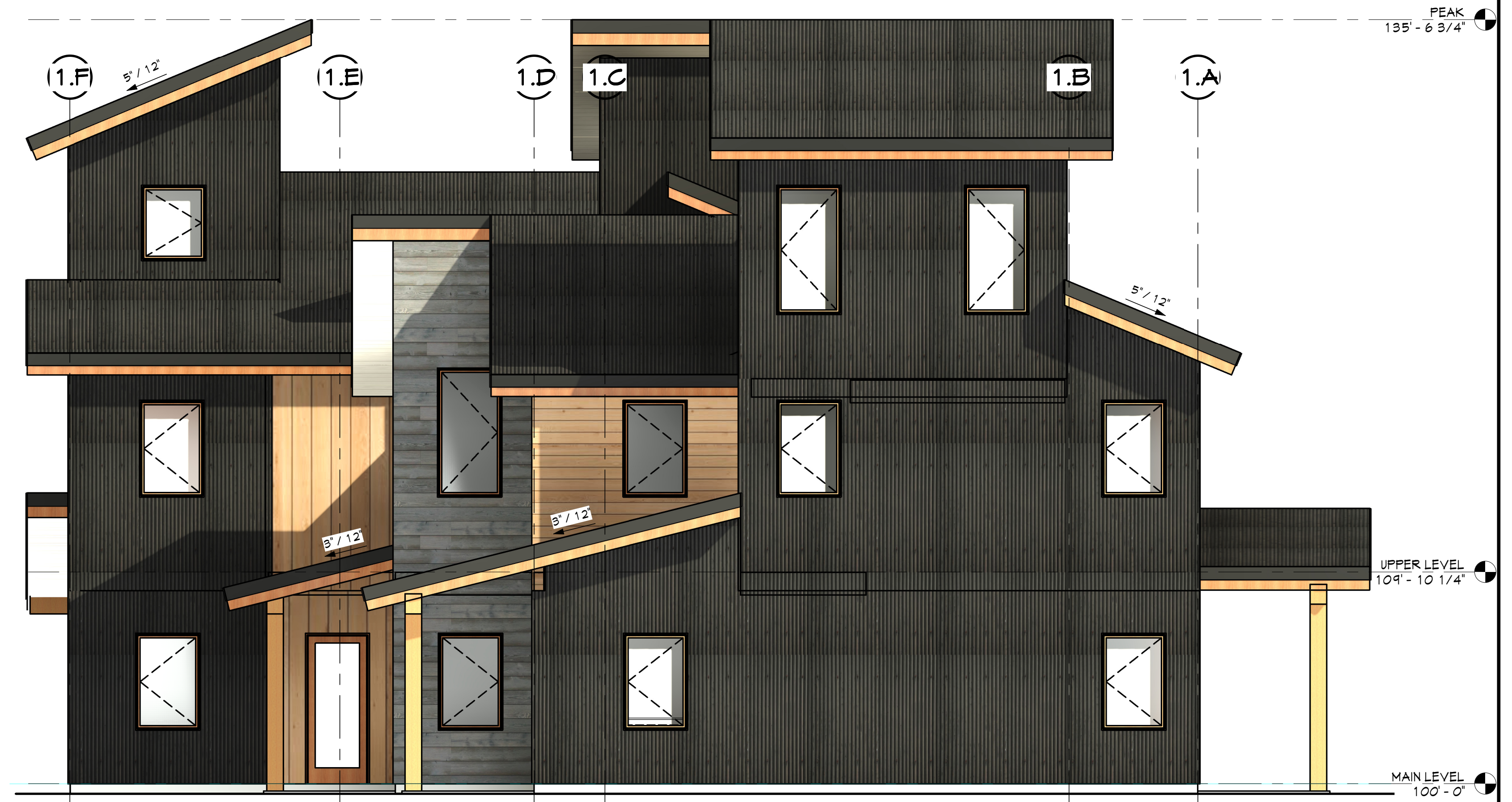
④ Elevation BD 1 SOUTHEAST 1/4" = 1'-0" (GLAZING = 15.0%)
