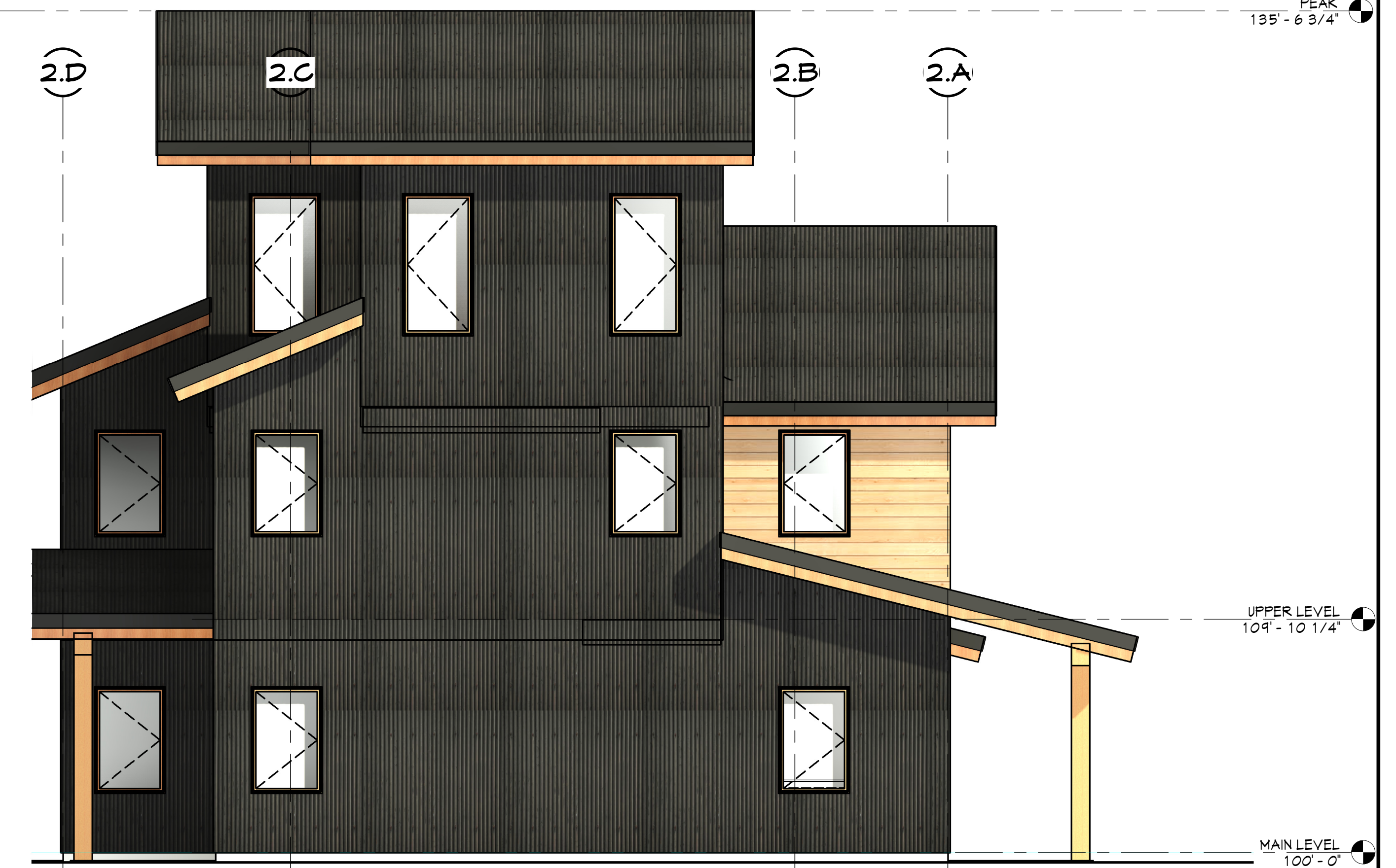
② Elevation BD2 SOUTHEAST 1/4" = 1'-0" (GLAZING = 14.2%)
