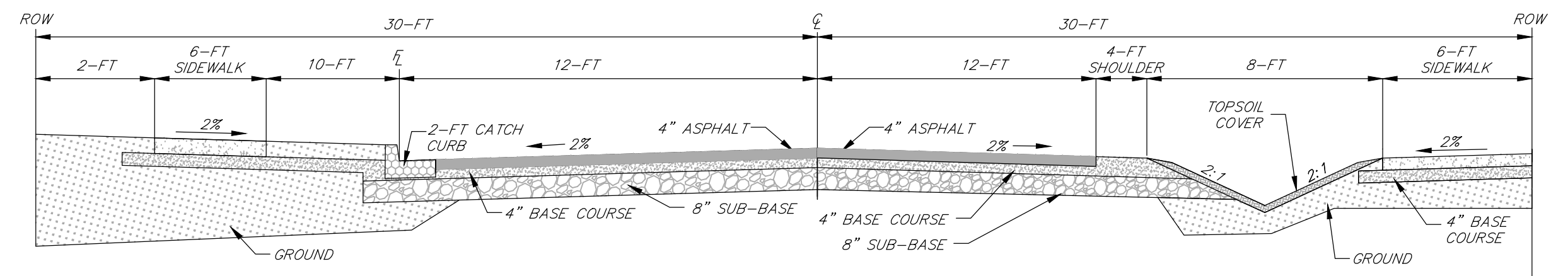
BRATTON DRIVE ROADWAY SECTION TO BE UTILIZED ON ENTIRE PROJECT N.T.S.
