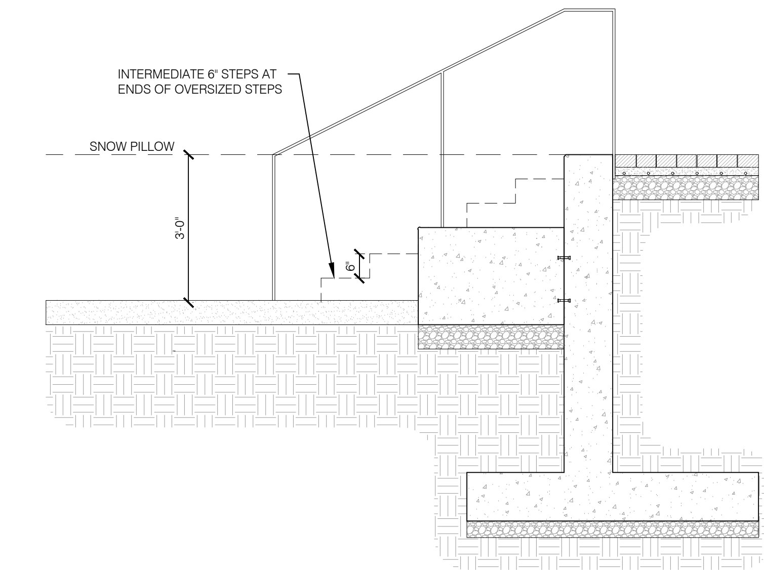
2 TYPICAL SNOW EDGE CONDITION 1/2" = 1'-0"
