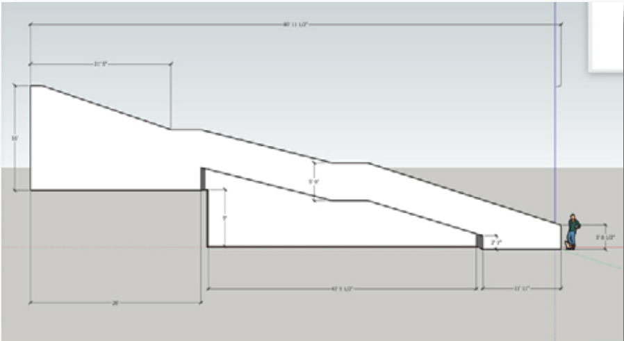
WALL DIMENSIONS
