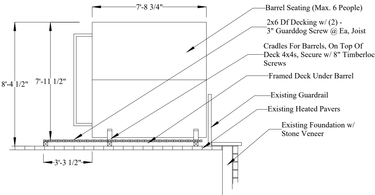
BARREL ELEVATIONS
