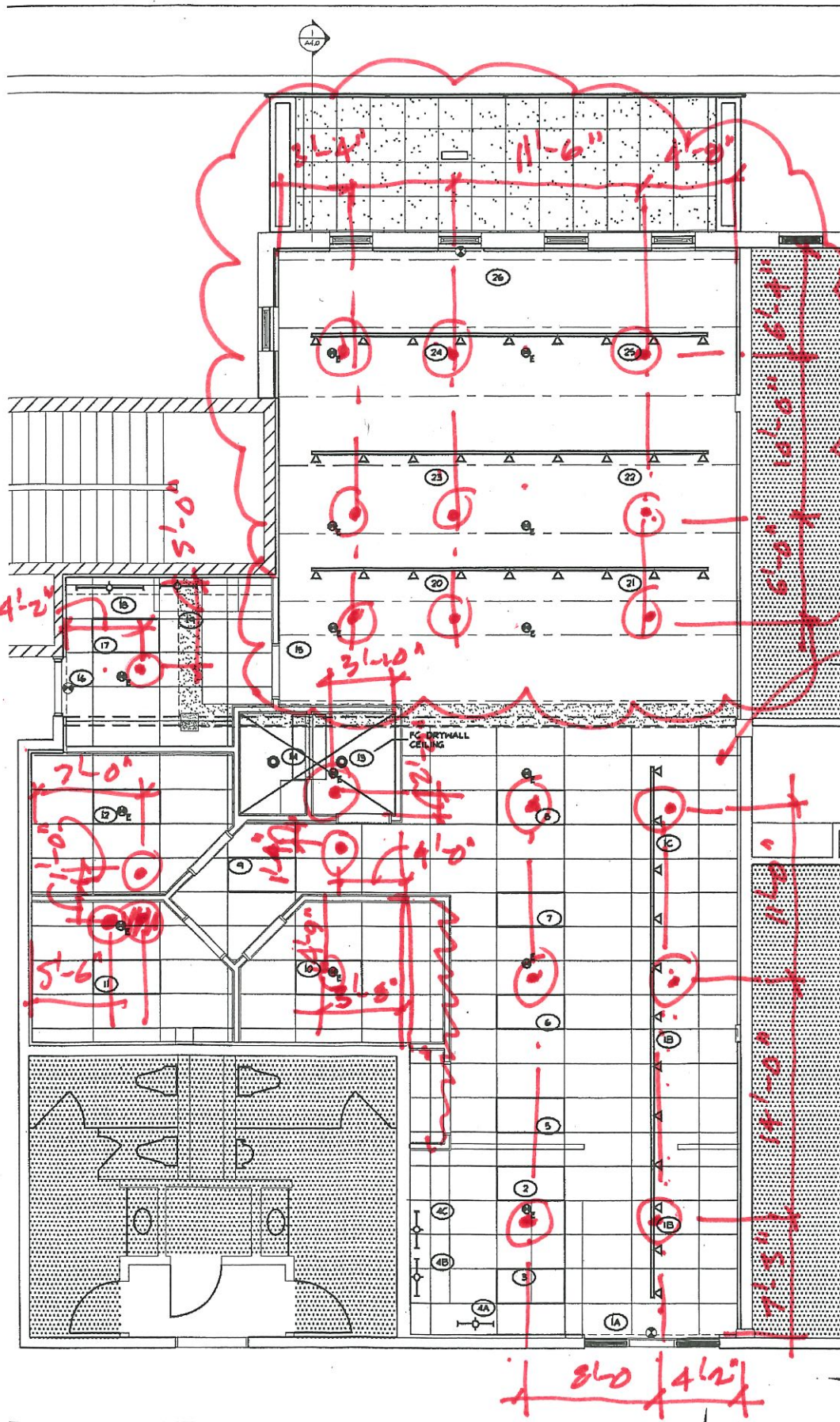
REFLECTED CEILING PLAN 4" = 1'-0" EE A2.0 OFFICE SPACE - 2,007 SF
