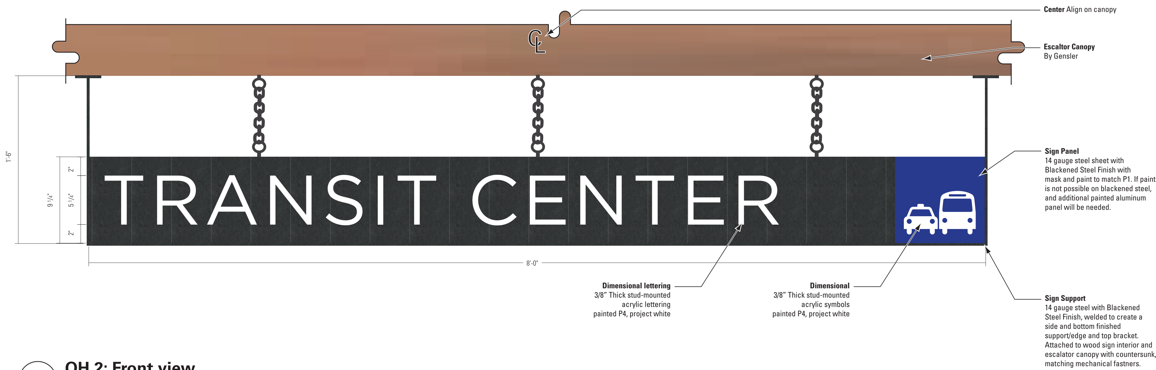
1 OH 2: Front view SCALE: 2" = 1'-0"
