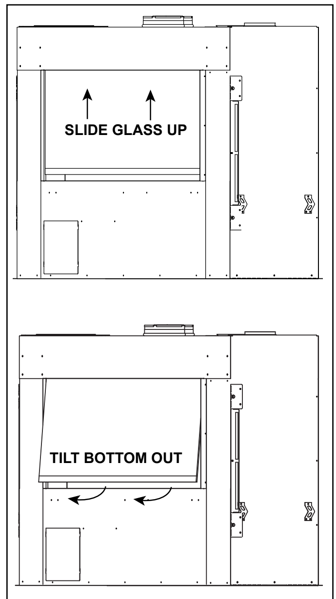
Figure 11.28 Barrier Glass Removal
