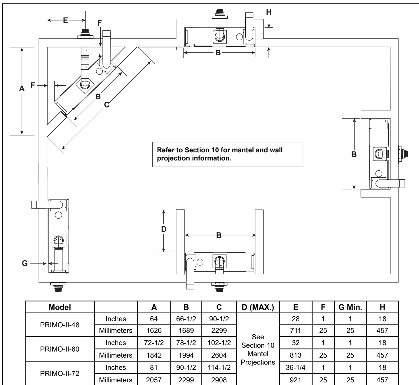
Figure 3.3 Appliance Locations PRIMO-II-48, PRIMO-II-60, PRIMO-II-72
