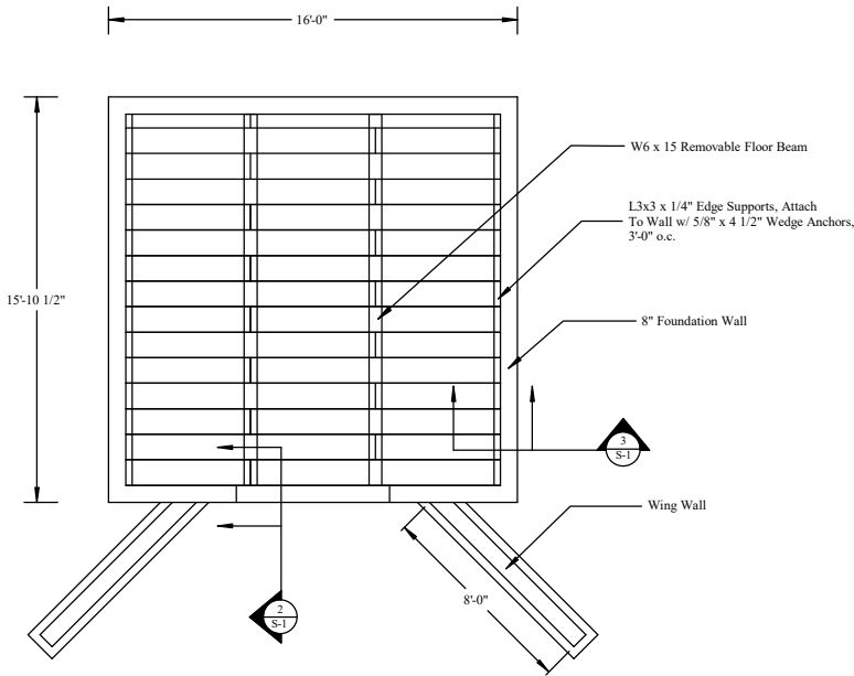
PLAN VIEW FLOOR SUPPORT
