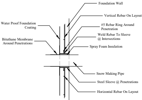
SECTION 1 S-1 SCALE: 1/2" = 1'-0" PIPE PENETRATION DETAIL
