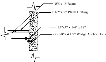
SECTION 2 S-1 Scale: 1/2" = 1' BEAM DETAIL
