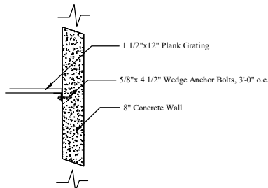
SECTION 3 S-1 Scale: 1/2" = 1' EDGE SUPPORT DETAIL
