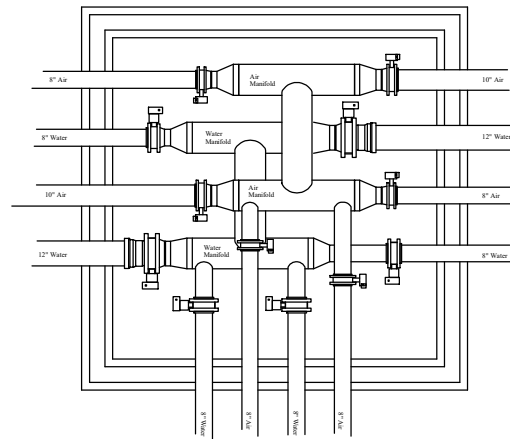
PIPE LAYOUT
